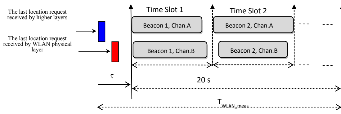
Figure 4.3.2.1.3-1: WLAN Measurement Time
