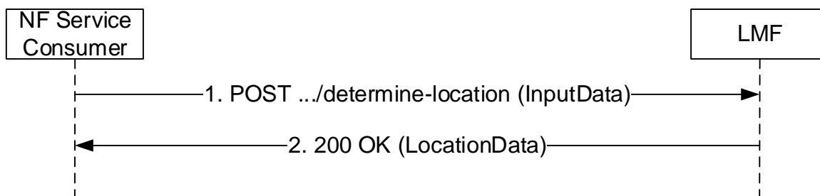
Figure 5.2.2.2.2-1: DetermineLocation Request
