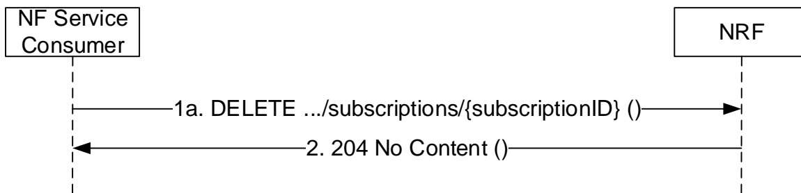
Figure 5.2.2.7.1-1: Unsubscription to Notifications
