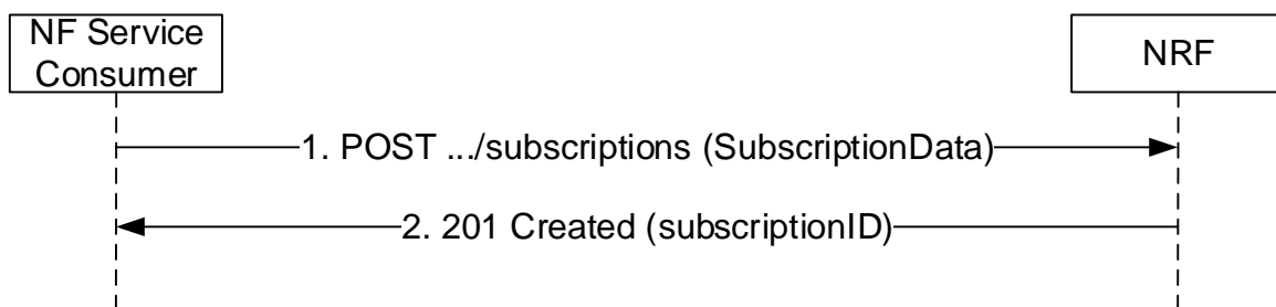
Figure 5.2.2.5.2-1: Subscription to newly registered NF Instances
