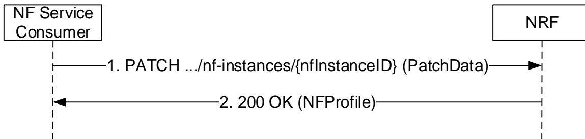
Figure 5.2.2.3.2-1: NF Heart-Beat
