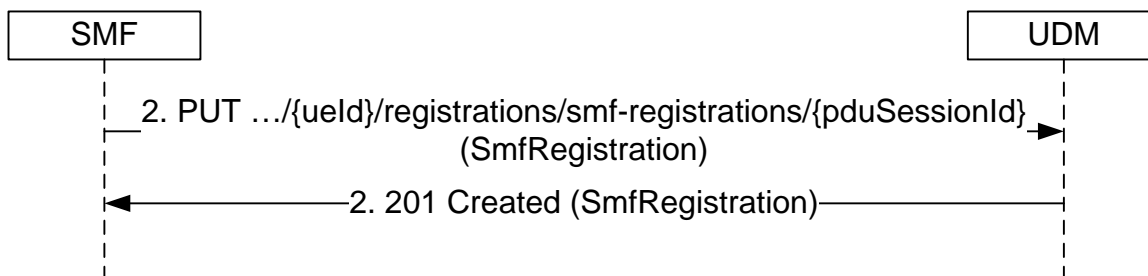
Figure 5.3.2.2.4-1: SMF registration
